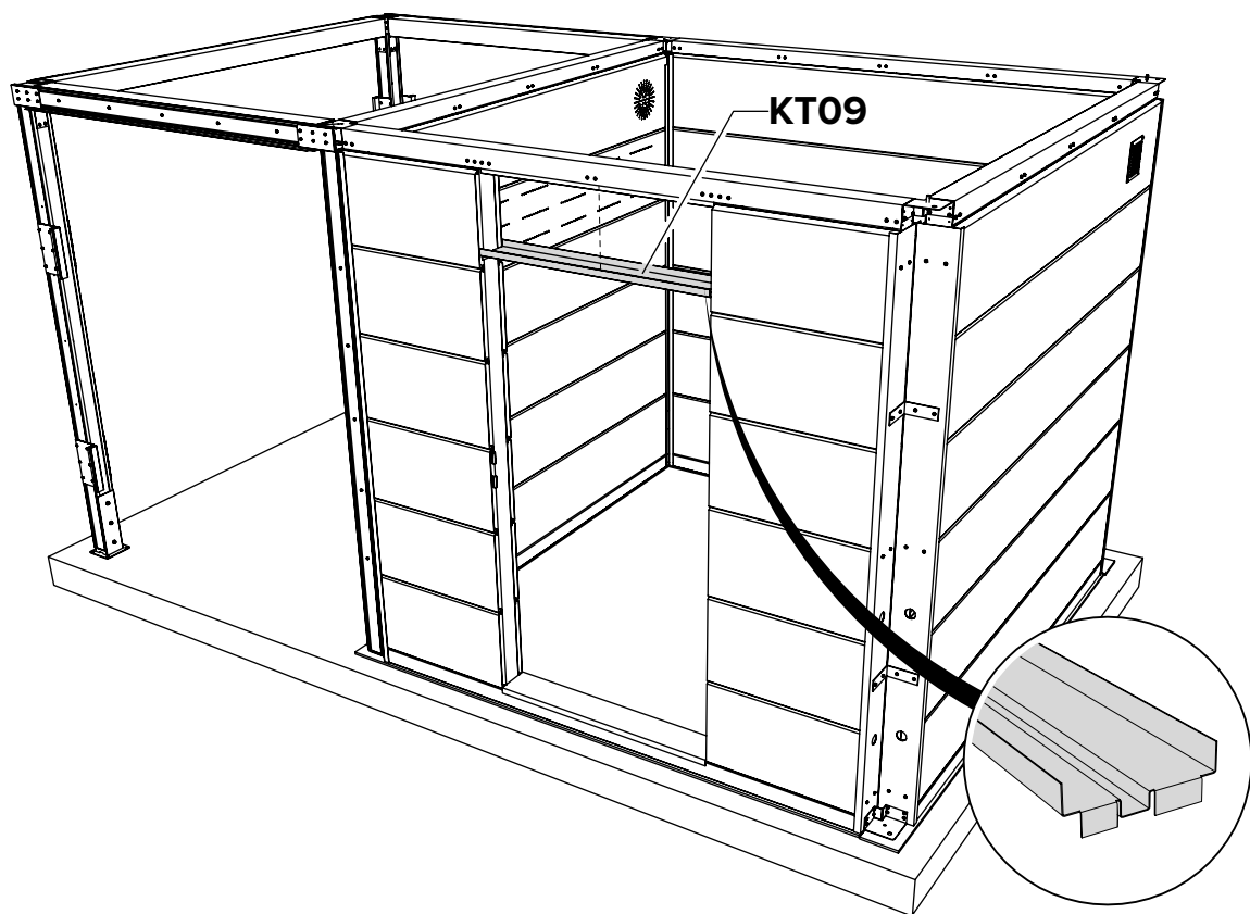
A Porta / Puerta
