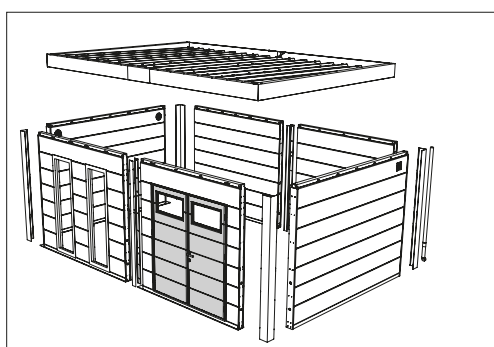
Porta / Puerta
